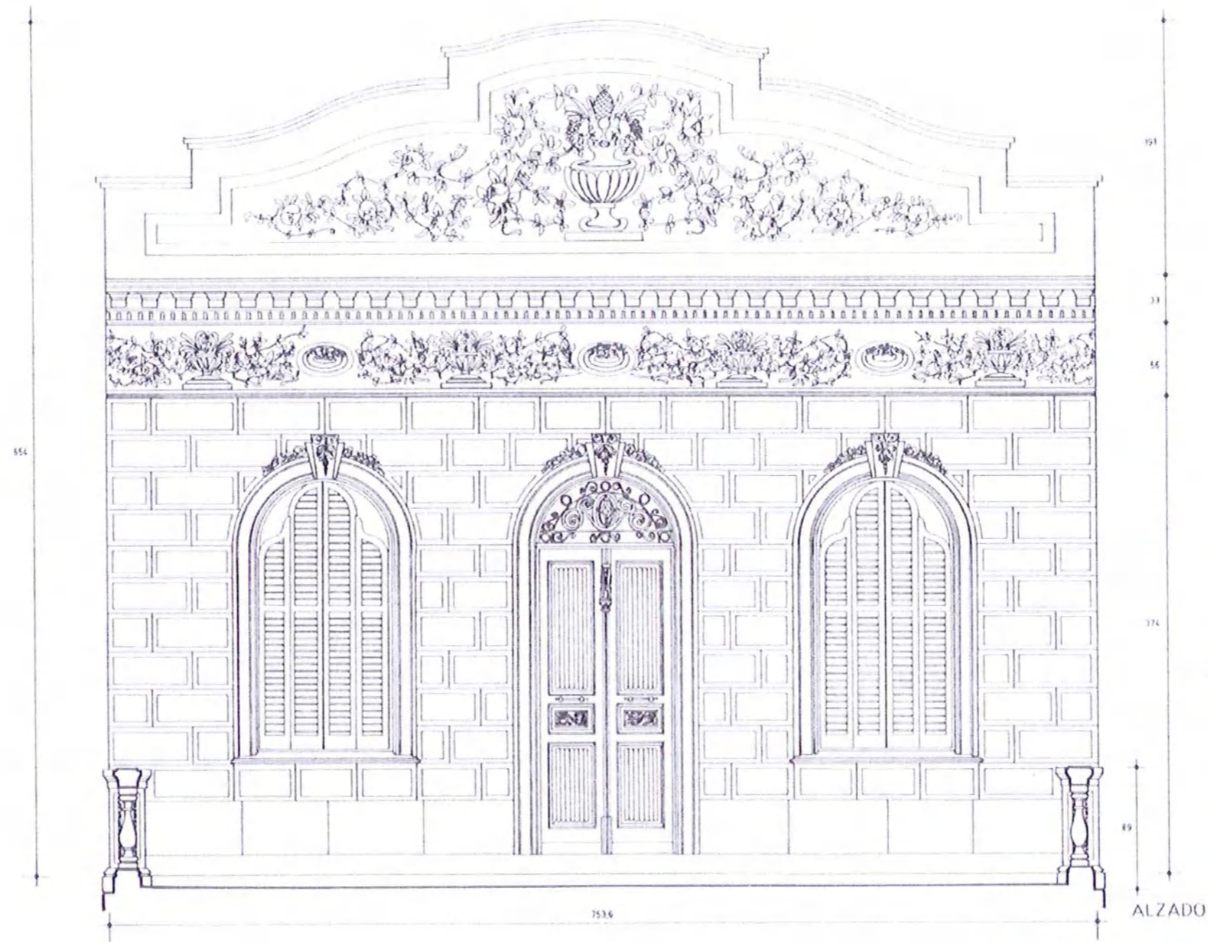
Façana Principal
